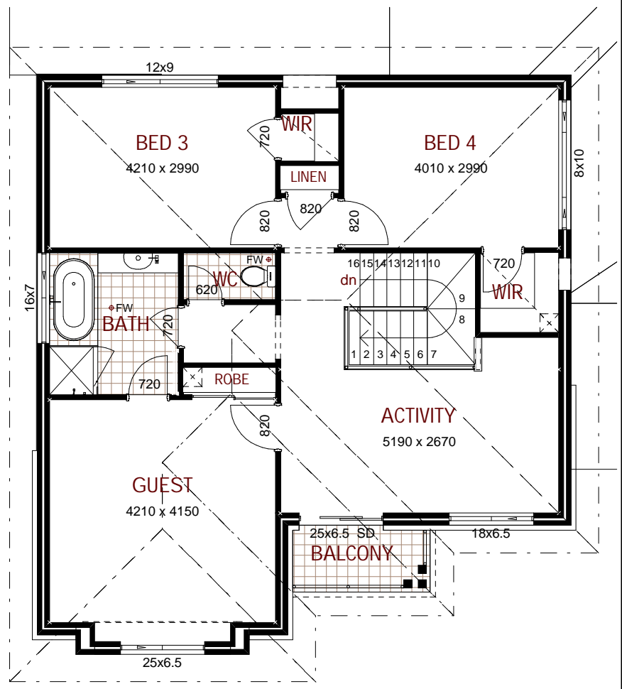
UPPER FLOOR PLAN 1:100
