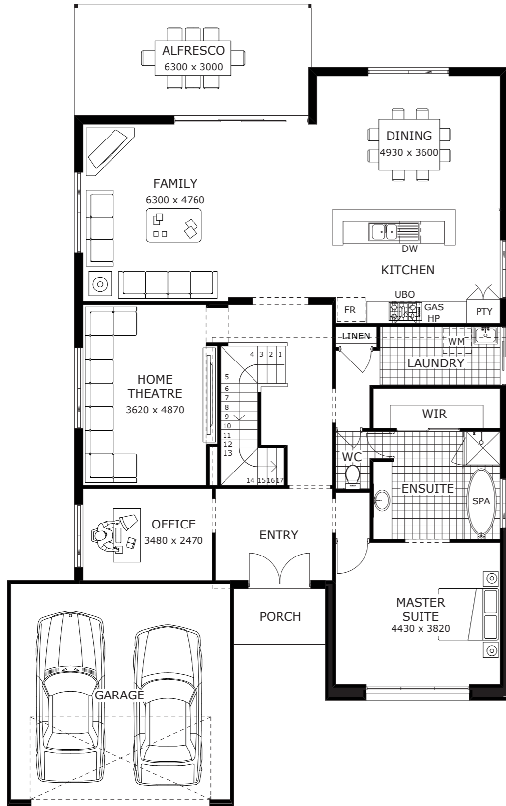
GROUND FLOOR
