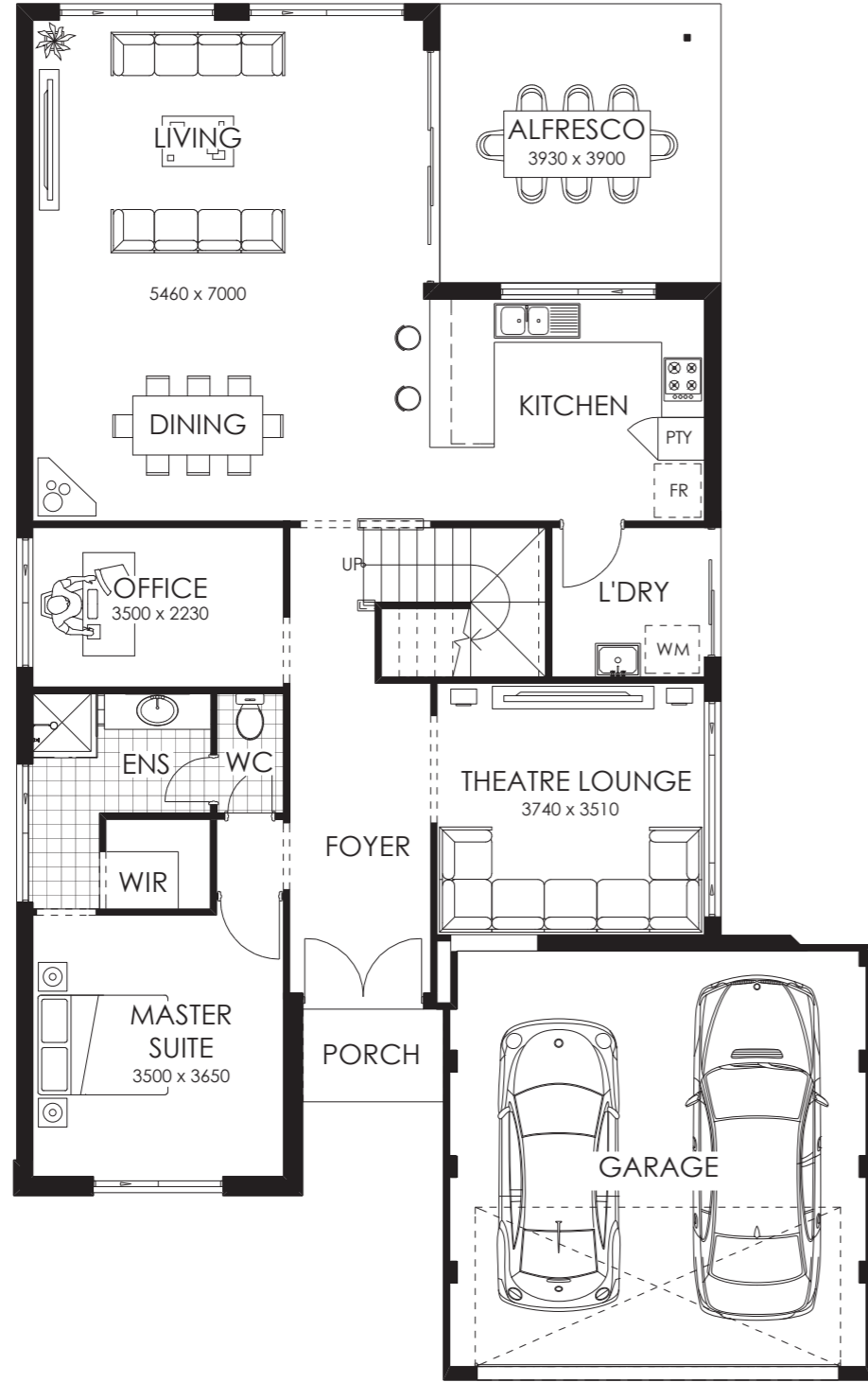
GROUND FLOOR
