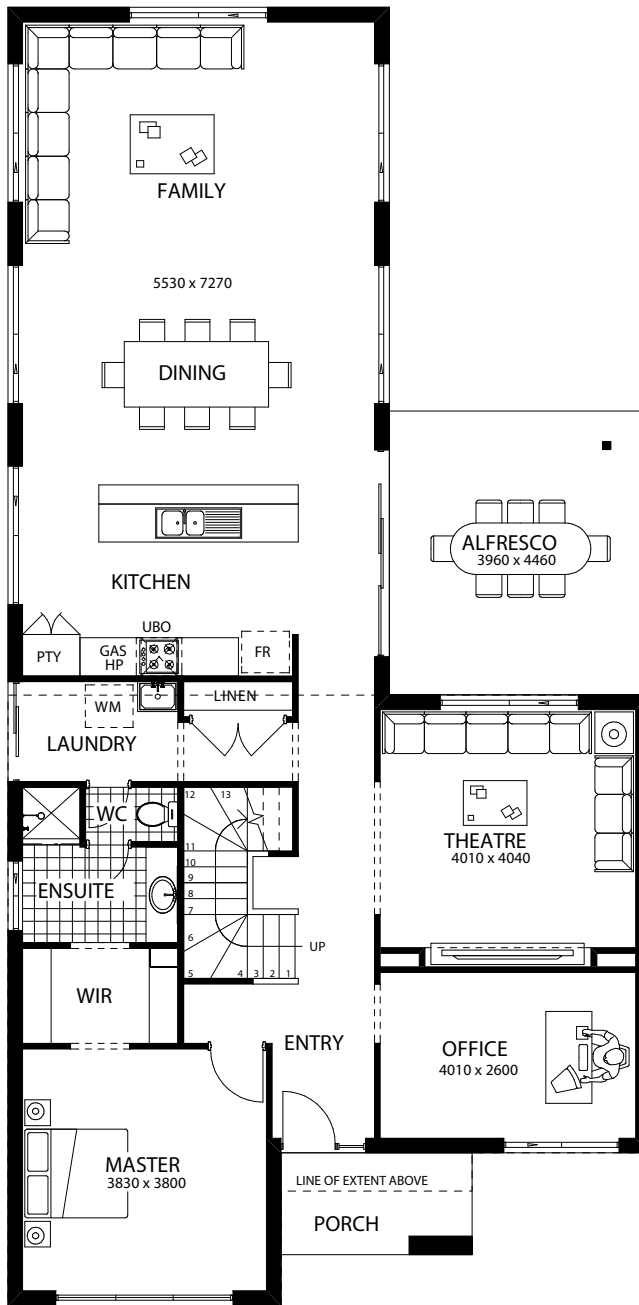
Ground Floor
