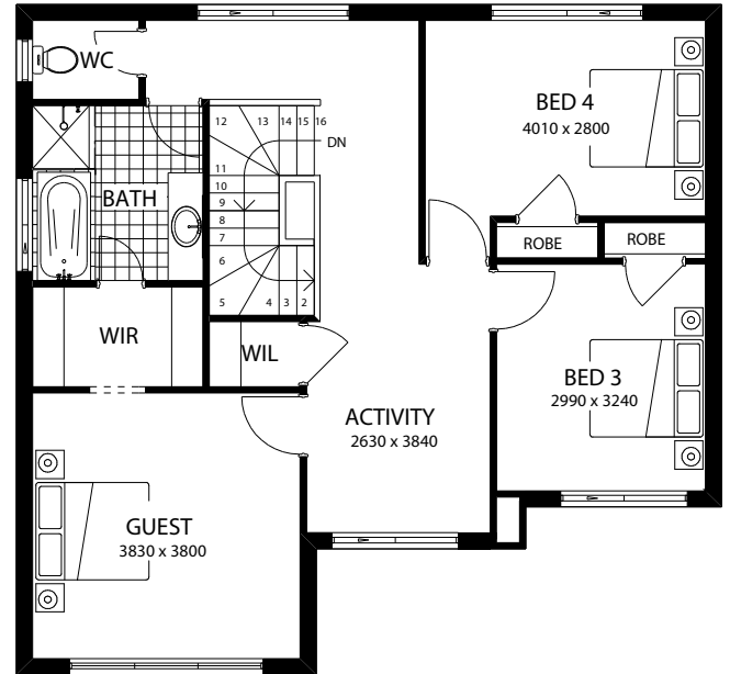
Upper Floor
