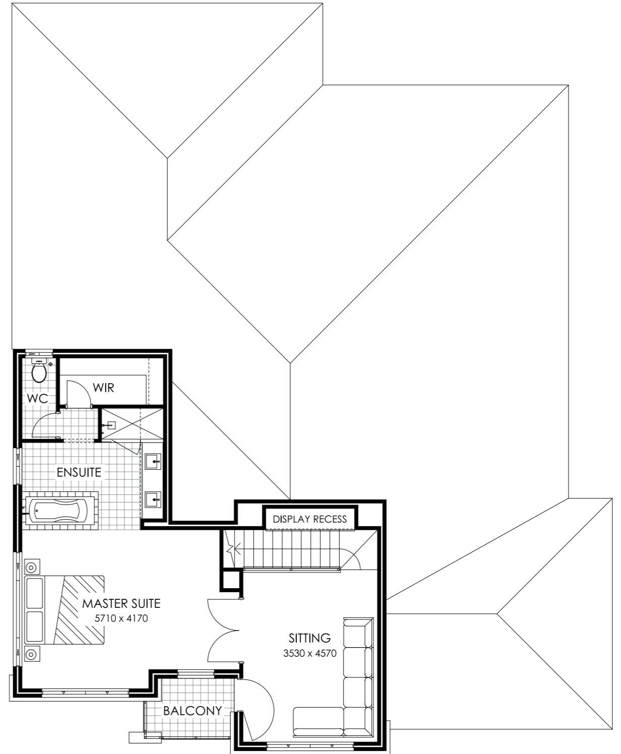
UPPER FLOOR PLAN
